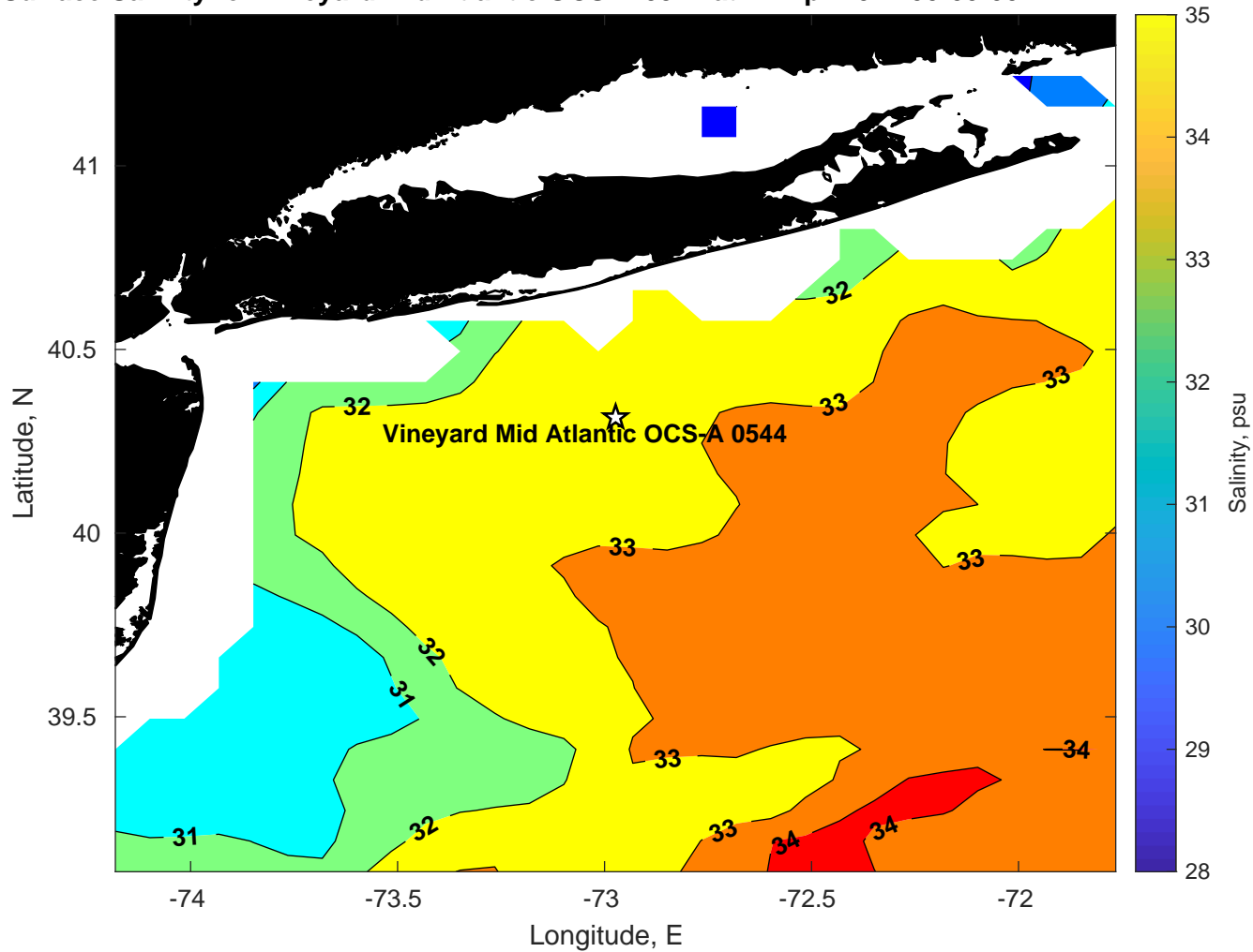
Surface Salinity for Vineyard Mid Atlantic OCS-A 0544 at 27-Apr-2024 00:00:00
